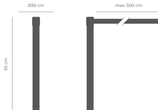
Poteau LIMIT Ech. 1:20 (Poids: 11kg)
