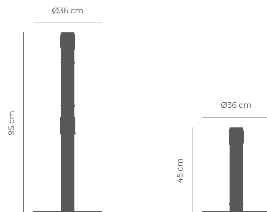
Poteau LIMIT DUAL Ech. 1:20 (Poids: 11Kg)
